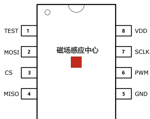
图 4: SOP-8 4.9mmx6mm
